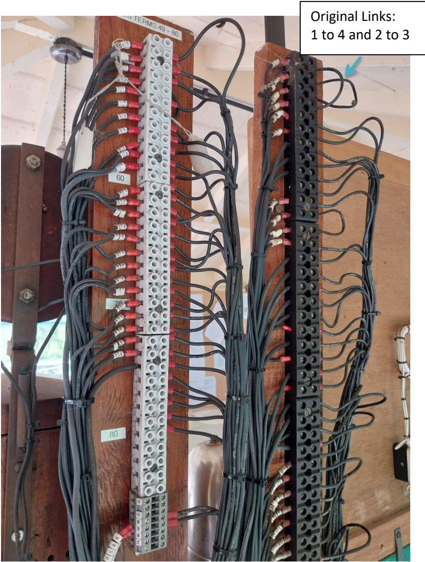
Original Wiring
